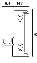
_Profilo superiore e inferiore/ Upper and lower profile
