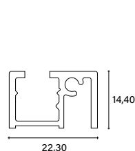
_Trafila walk-in/ Walk-in profile
