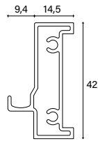
_Profilo superiore e inferiore/ Upper and lower profile
